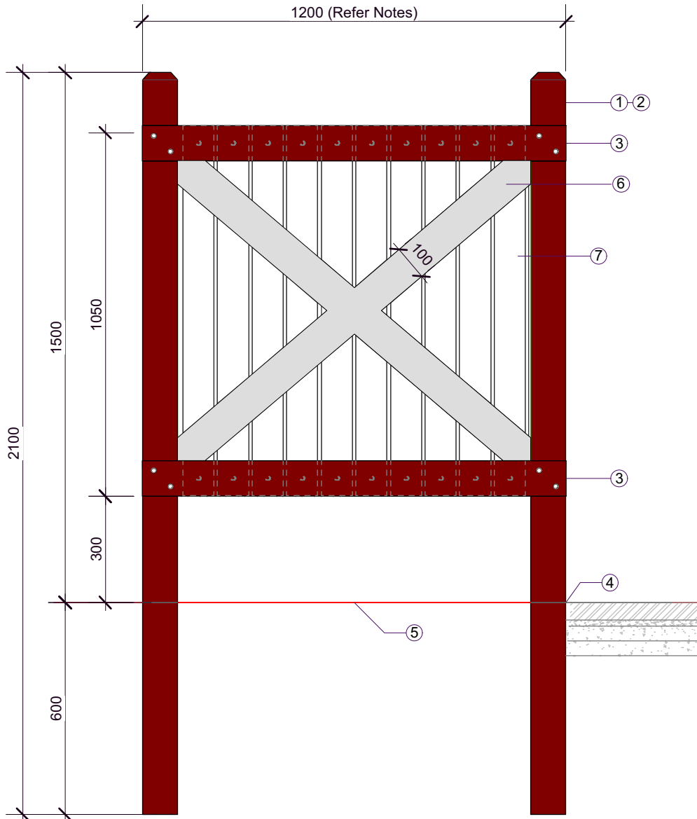
1 CTG : FRONT ELEVATION 1:25 at A4
