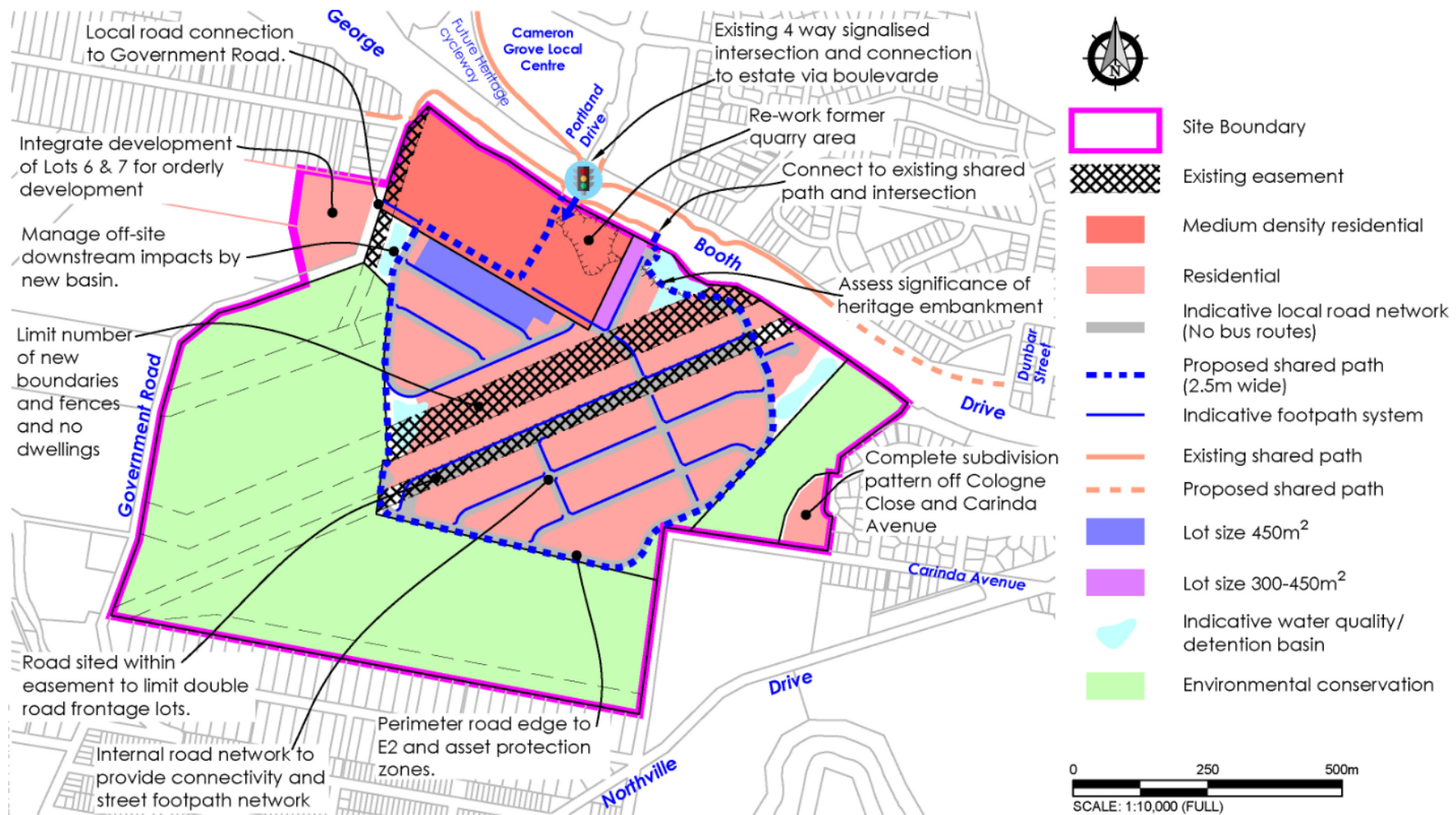
Figure 2 - Edgeworth Area 3 - Indicative Structure Plan
