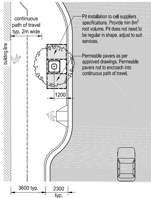
D2 Single tree in pit plan view 1:200
