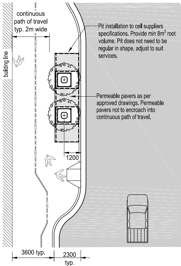
D1 Multiple trees in linked pit plan view 1:200
